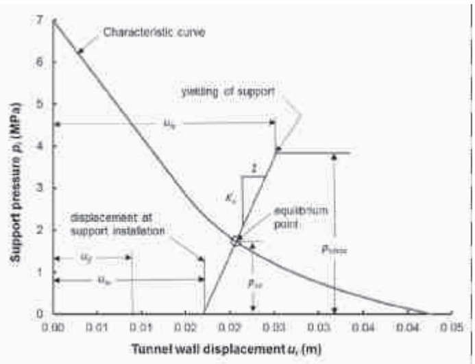
Figure 2 Rock Support Interaction in Tunnels
